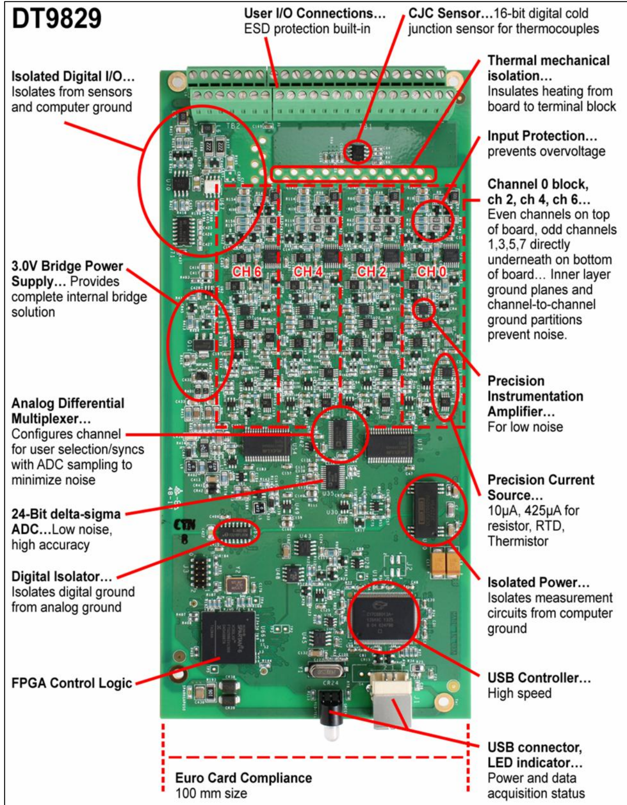
Figure 5. Every design factor is presented to show the uncompromised, high-integrity performance built into the OEM embedded version.
