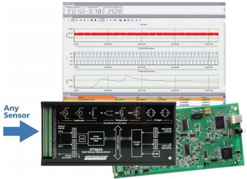
Figure 1. The DT9829 provides up to 8 multi-sensor input channels. Any sensor merely has to be connected at an input and all selections, including any necessary for excitation, cold junction compensation or bridge completion, are included and supported by QuickDAQ. No other circuitry or external components are necessary. OEM model (no enclosure) for embedding is available.
